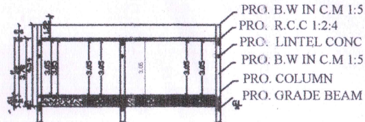
SECTION ON A A
