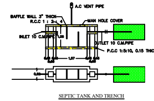
Septic Tank
