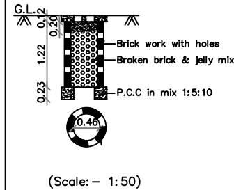
PERCOLATION PIT FOR 30 Sq. m.
