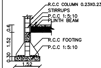
COLUMN DETAILS
