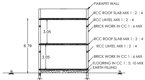
SECTION ON AB & ( HALF ELEVATION)
