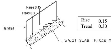
STAIRCASE DETAIL
