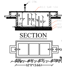
SECTION PLAN SEPTIC TANK DETAILS
