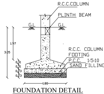
FOUNDATION DETAIL
