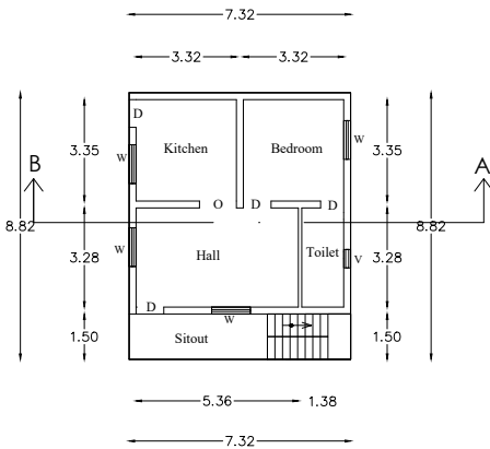
PRO GROUND FLOOR PLAN
