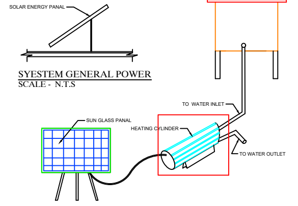
SOLAR WATER HEATING SYSTEM SCALE - N.T.S
