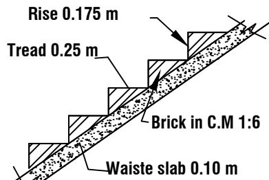
STAIR DETAILS
