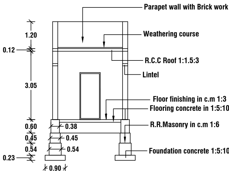
SECTION ON CD
