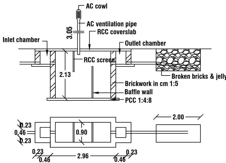
SEPTICTANK DETAILS
