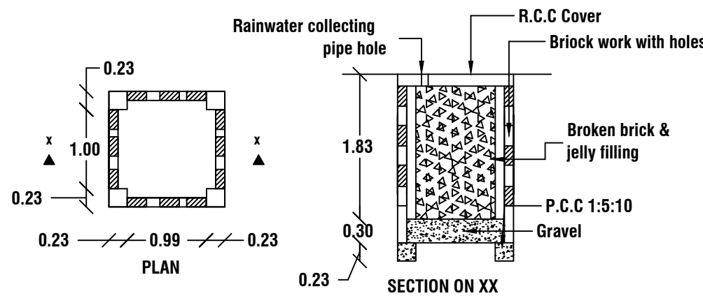
RAINWATER HARVEST WELL
