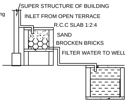
RAINWATER HARVESTING
