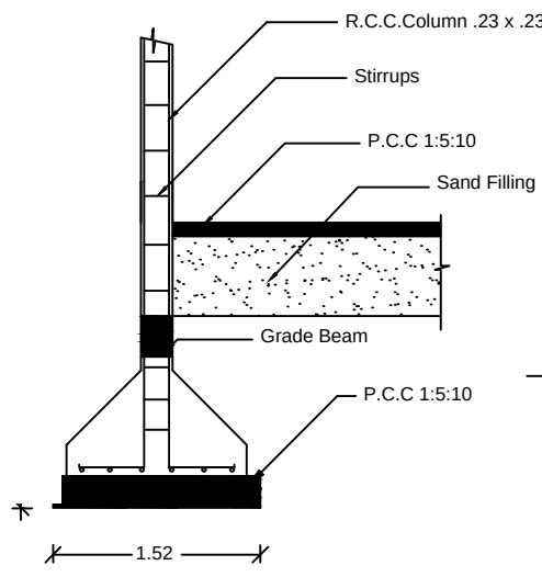
COLUMN DETAIL
