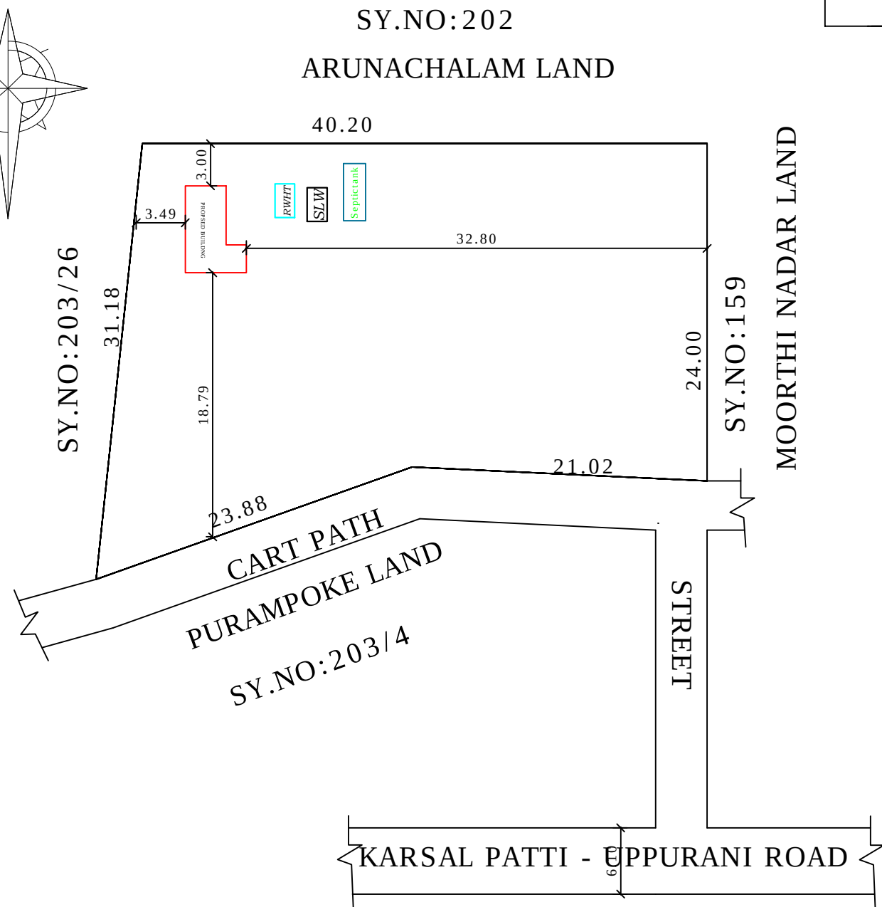
SITE PLAN
