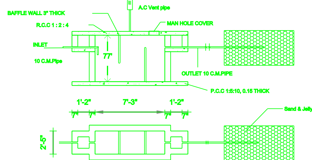
Septic tank and trench
