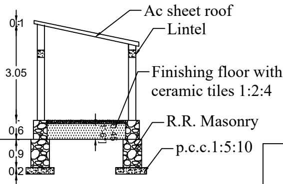
SECTION AB
