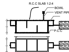
SEPTIC TANK AND TRENCH NTS
