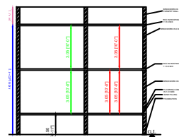
SECTION ON AA
