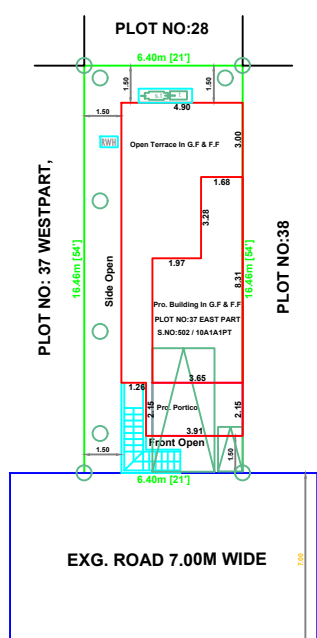
SITE PLAN (SCALE 1:100)
