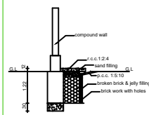
PLINTH BOUNDARY PERCOLATION PIT
