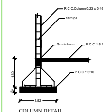
COLUMN DETAIL
