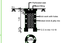
PERCOLATION PIT FOR 30 Sq. m. (Scale:- 1:50)
