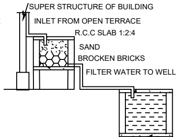
RAINWATER HARVESTING
