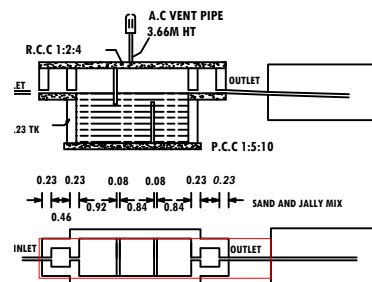
SEPTIC TANK AND TRENCH (EXISTING)
