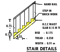
STAIR DETAILS
