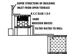
DETAILS OF FILTER BED & WELL
