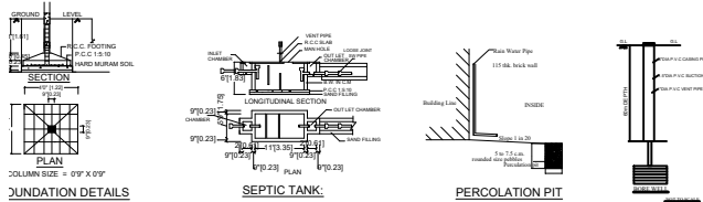
FOUNDATION DETAILS
