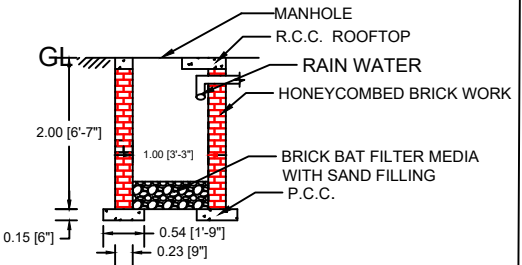
SECTION ON O - P
