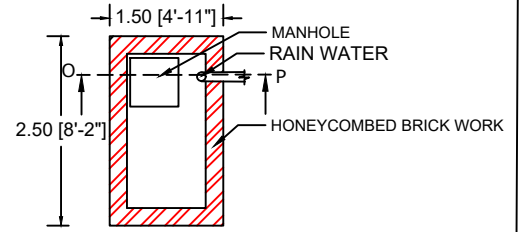
PLAN RAIN WATER HARVESTING
