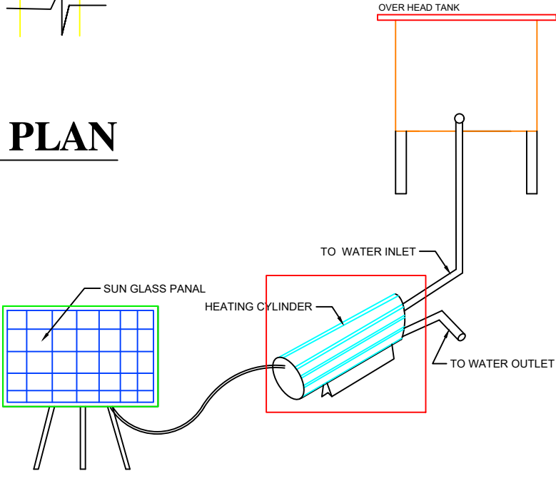
SOLAR WATER HEATING SYSTEM SCALE - N.T.S
