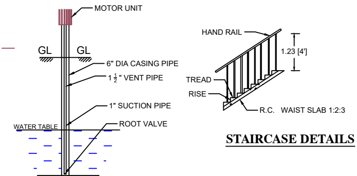
SEC.OF BOREWELL
