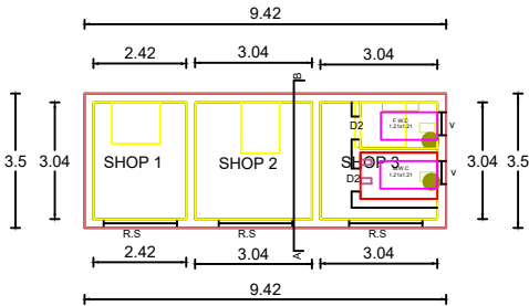
GROND FLOOR PLAN
