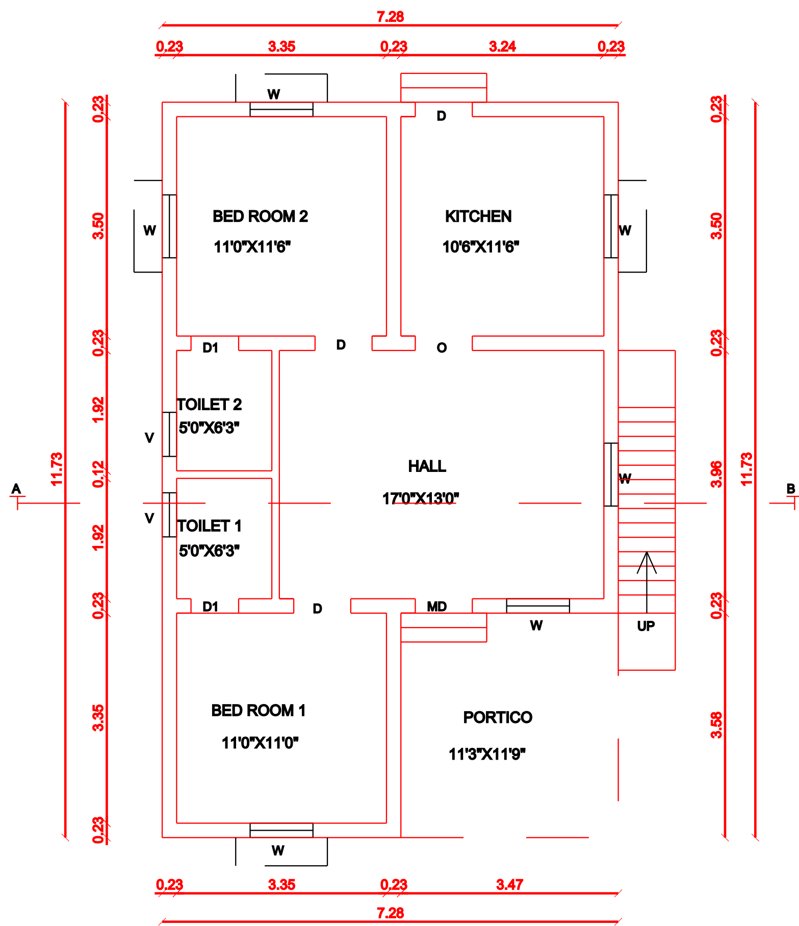
ND FLOOR PLAN
