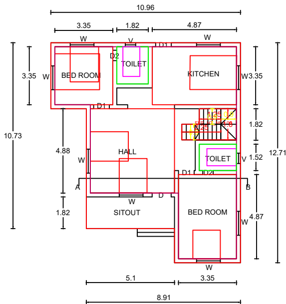
GROND FLOOR PLAN
