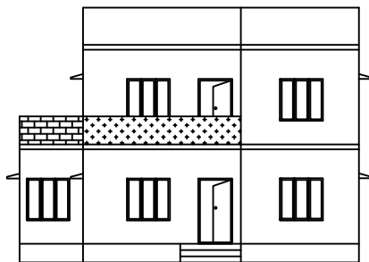
FRONT ELEVATION
