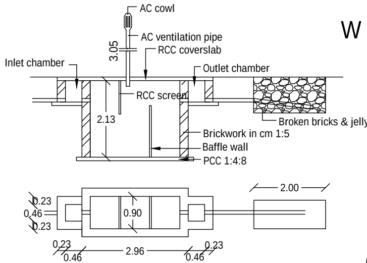
SEPTICTANK DETAILS
