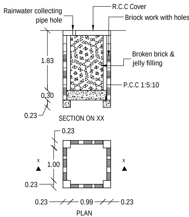
RAINWATER HARVEST WELL
