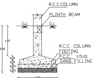
FOUNDATION DETAIL
