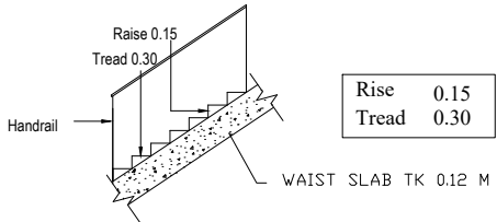
STAIRCASE DETAIL
