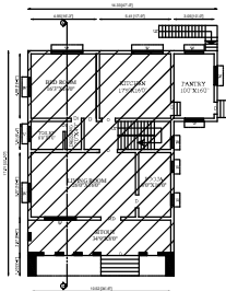
REVISED GROUND FLOOR PLAN
