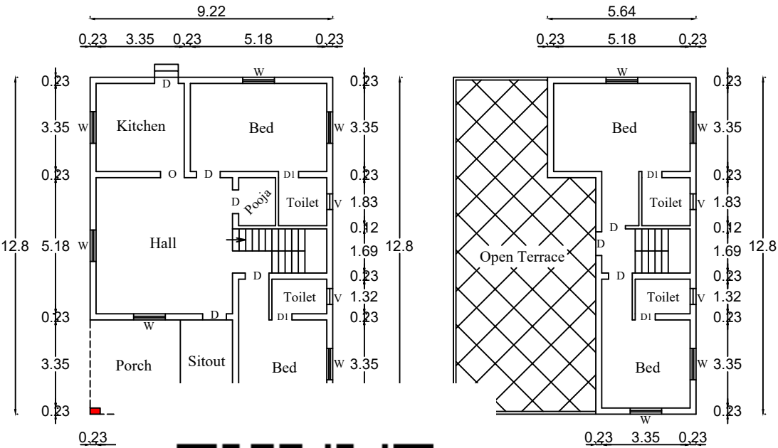
RST FLOOR PLAN
