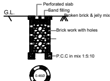
PERCOLATION PIT FOR 30 Sq. m.
