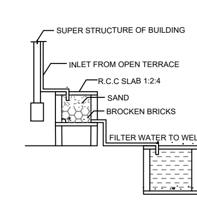
DETAILS OF FILTER BED & WELL
