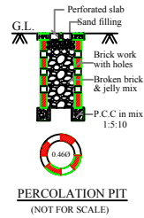
Rainwater harvesting
