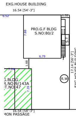
F PLAN SCALE 1:200
