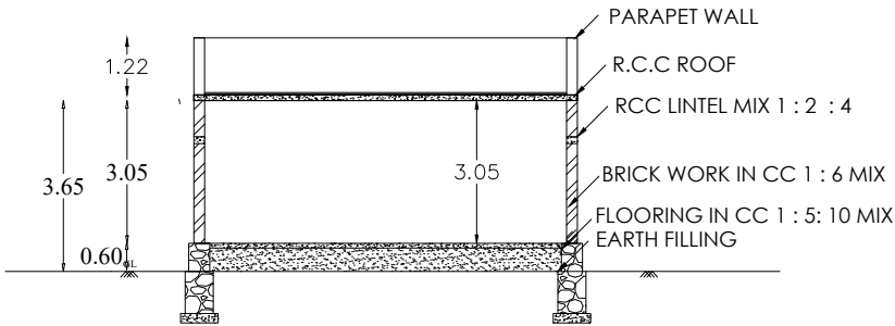
SECTION ON AB & ( HALF ELEVATION)
