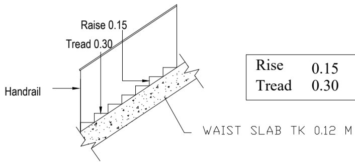
STAIRCASE DETAIL
