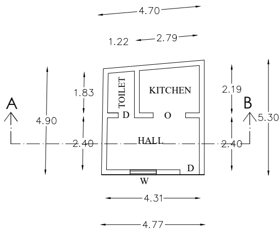
PRO GROUND FLOOR PLAN
