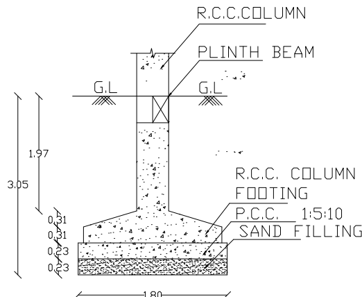
FOUNDATION DETAIL
