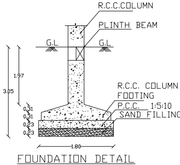
FOUNDATION DETAIL
