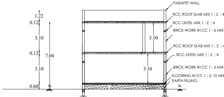
SECTION ON AB & (HALF ELEVATION)
