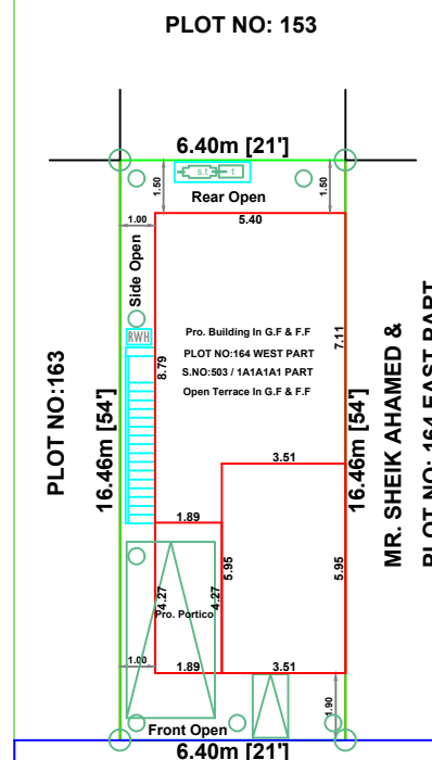
R.11, EXG. ROAD 7.00M WIDE
