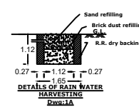
DETAILS OF RAIN WATER HARVESTING Dwa:1A
