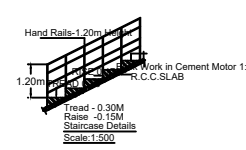
Staircase Details Scale:1:500
