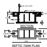
SEPTIC TANK PLAN
