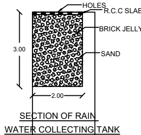
SECTION OF RAIN WATER COLLECTING TANK
