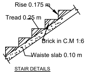
STAIR DETAILS
