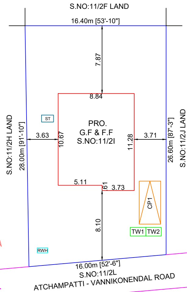
SITE PLAN
