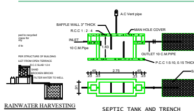
RAINWATER HARVESTING
