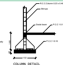
COLUMN DETAIL
