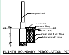
PLINTH BOUNDARY PERCOLATION PIT
