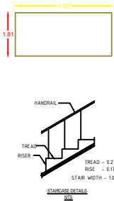
STAIRCASE DETAILS
