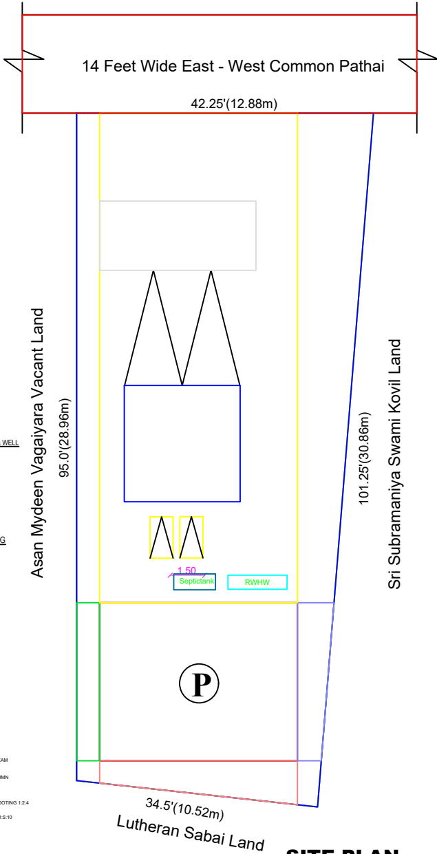
SITE PLAN
