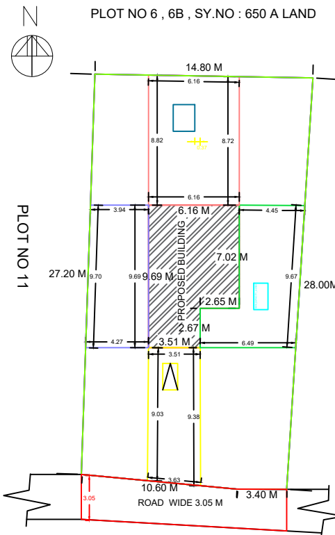
Site Plan 1: 100 scale
