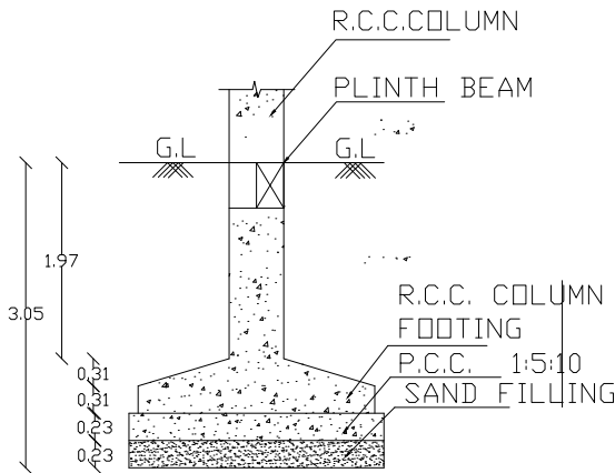
FOUNDATION DETAIL
