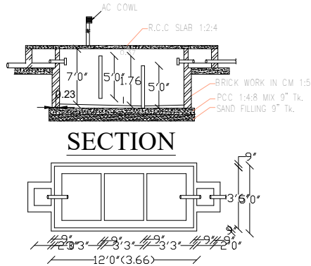
PLAN SEPTIC TANK DETAILS
