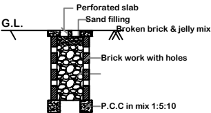
RAINWATER HARVESTING
