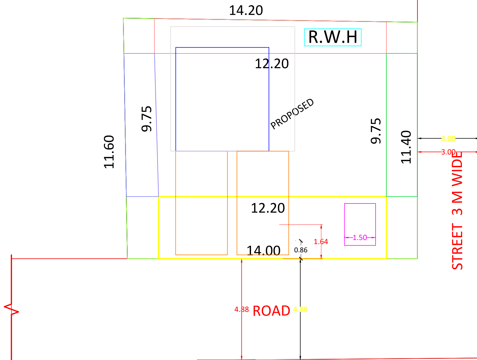
SITE PLAN
