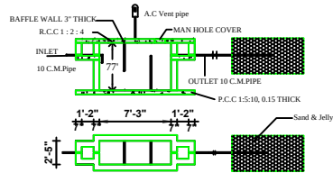
Septic tank and trench
