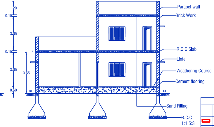
CROSS SECTION ON 'AB'
