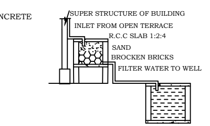
RAINWATER HARVESTING
