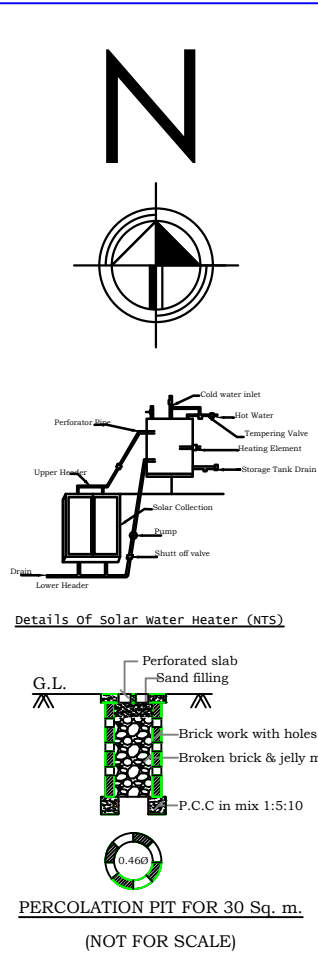
RAINWATER HARVESTING
