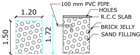
PLAN & SECTION OF RAIN WATER COLLECTION TANK
