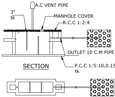
PLAN OF SEPTIC TANK & TRENCH
