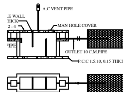
SEPTIC TANK & TRENCH
