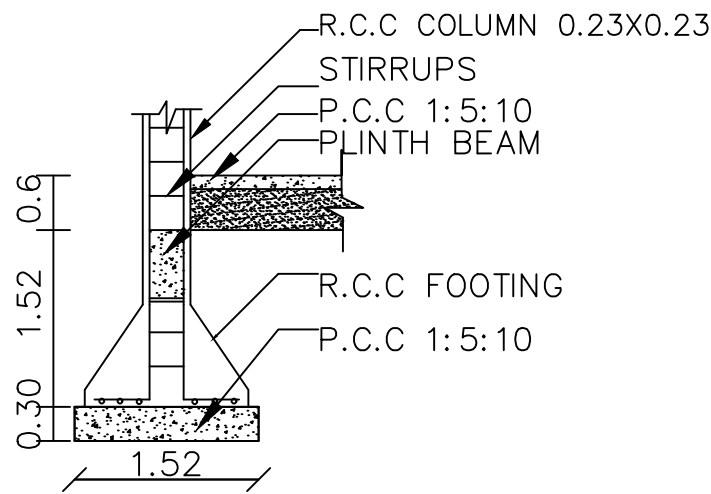
COLOUMN DETAILS
