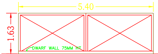
MAIN GATE
