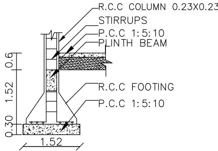
COLOUMN DETAILS
