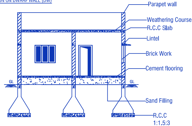
CROSS SECTION ON 'AB'
