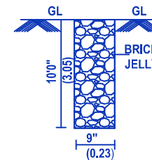
PERCOLATION PIT
