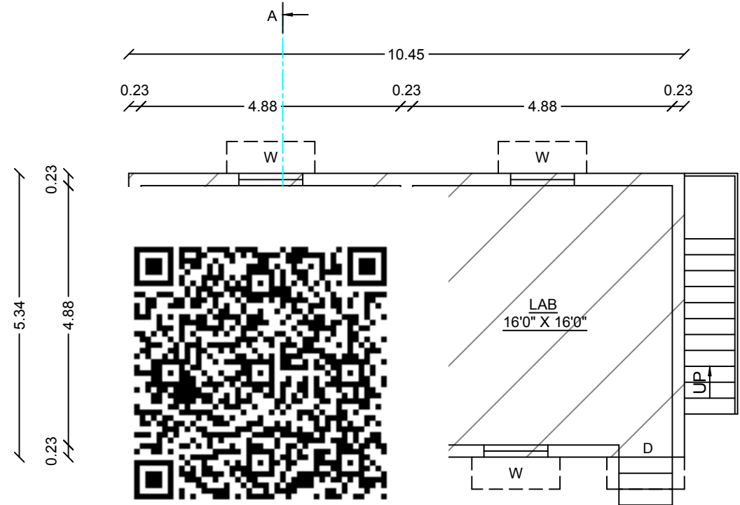
EXG. GROUND FLOOR PLAN
