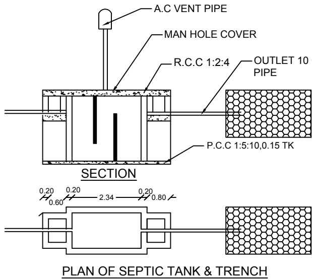
PLAN OF SEPTIC TANK & TRENCH
