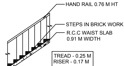
STEP DETAILS
