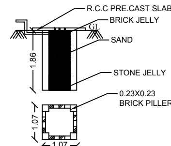
PLAN AND SECTION OF RAINWATER COLLECTION WELL
