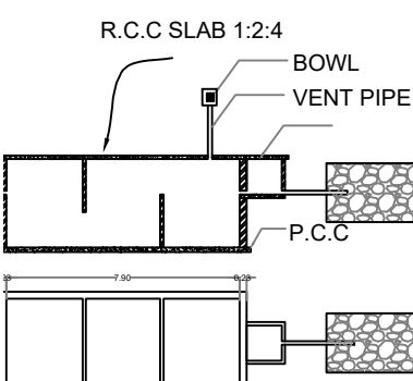
TIC TANK AND TRENCH NTS
