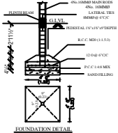
FOUNDATION DETAIL
