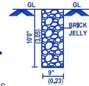
PERCOLATION PIT
