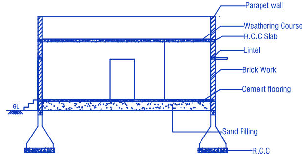
CROSS SECTION ON "AB"
