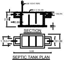
SEPTIC TANK PLAN
