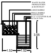
RECYCLING OF WASTE WATER FROM KITCHEN & BATHROOM
